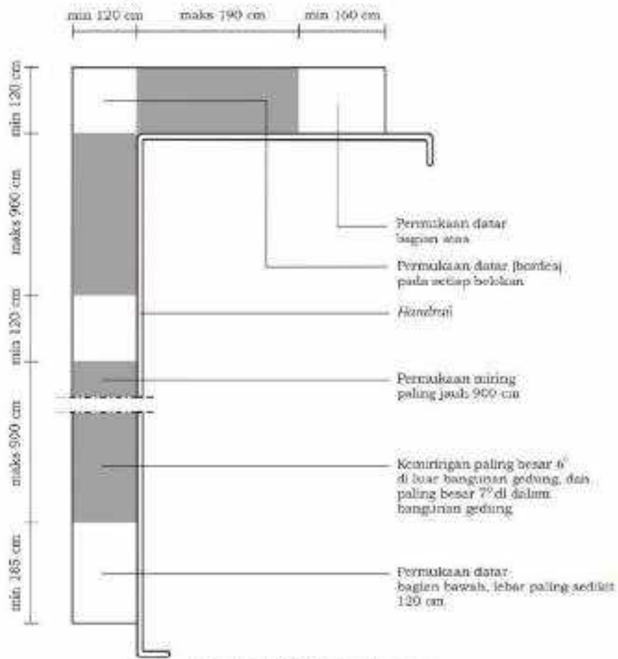
Gambar II.133. Pengecatan rana
