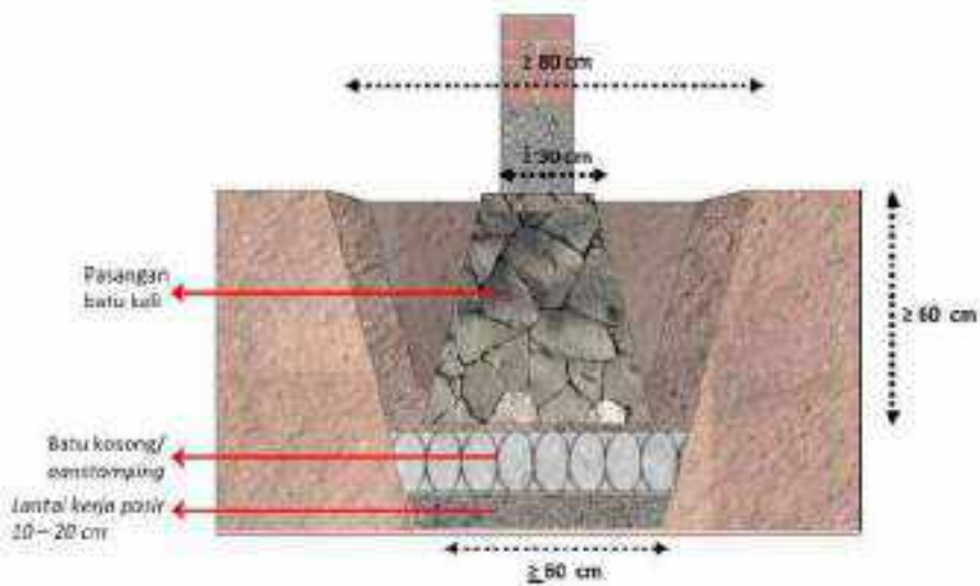
Gambar II.376 Pondasi
