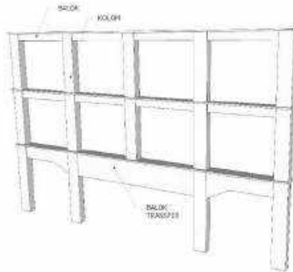
Gambar II. 20 Balok Transfer
