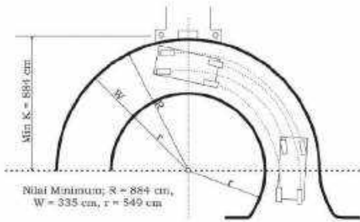
Gambar II.260 Kurva melingkar
