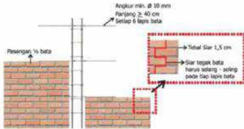
Gambar B.399 Detail Dinding
