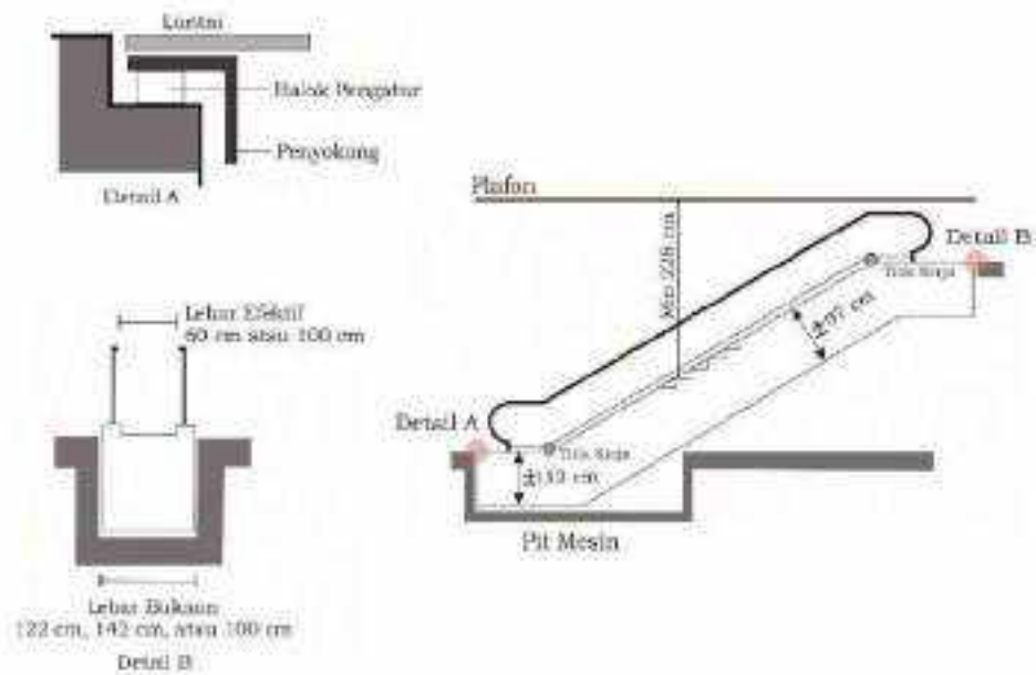
Gambar II.150. Detail eskalator
