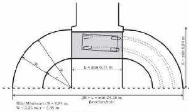
Gambar II.262 Kurva campuran
